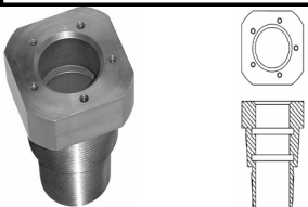
Threaded Adapter Fits 1-1/2" & 2" NPT Couplings
